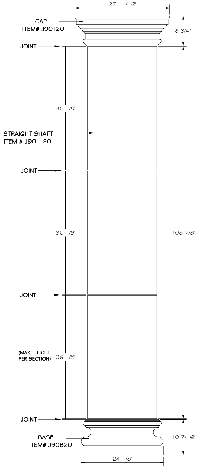
FRONT VIEW
