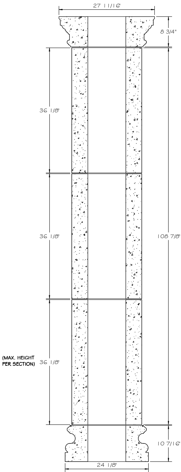
SECTION
