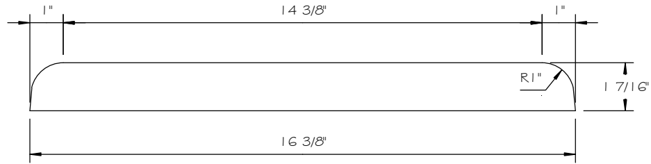
FRONT VIEW
