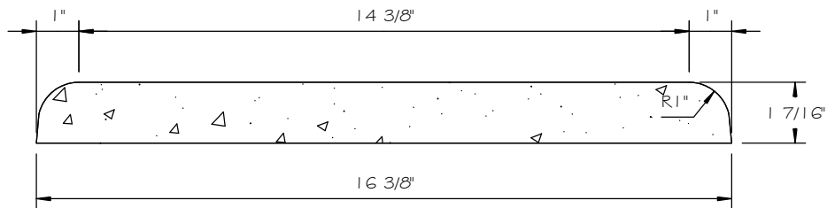
SECTION
