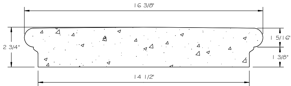
SECTION
