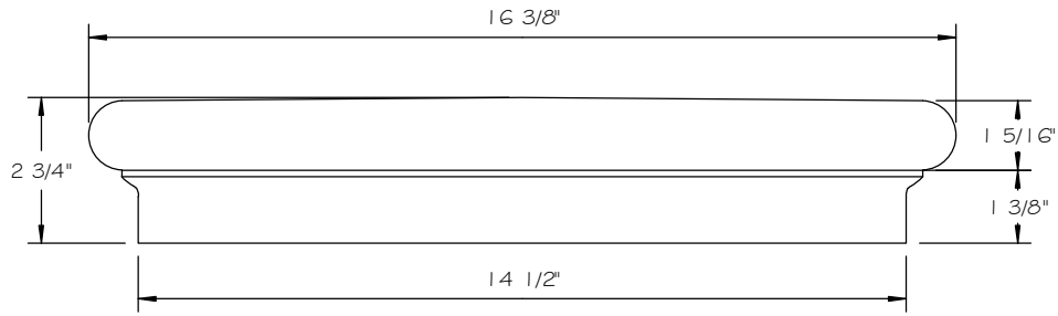
FRONT VIEW
