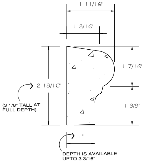
SECTION SCALE 6" = 1' 0"
