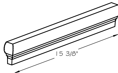
ISOMETRIC VIEW (LEFT RETURN SHOWN) NOT TO SCALE
