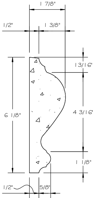
SECTION SCALE 4" = 1' 0"
